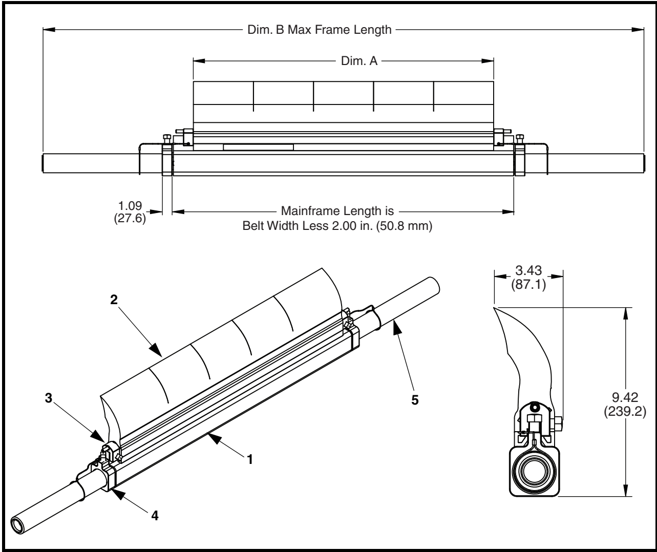
Figure 4. Martin® QC1+™ Cleaner HD Assembly, P/N C1QCHSXXXSXXXPX
